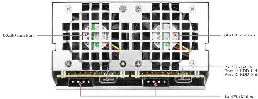
Rear view (iS2880-8S-S2D)
