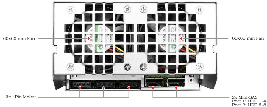
Rear view (iS2880-8S-U5D)
